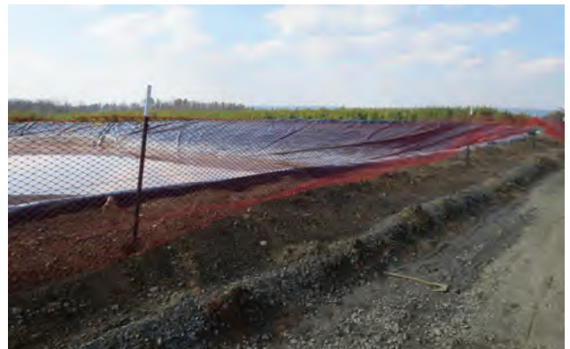
Above: Produced water storage pit. (Source: U.S. EPA)
